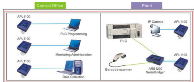
APL1100 UltraSpeed™ PowerLine Ethernet NetBridge™ — Wall Electrical Power line — Cat. 5 Cable RS232 Serial
