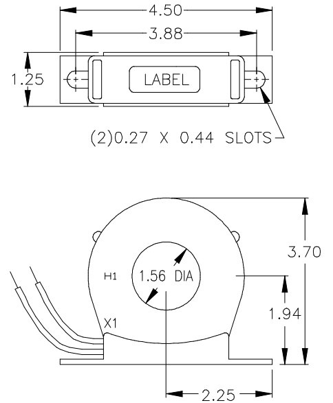
Model 5RBL
